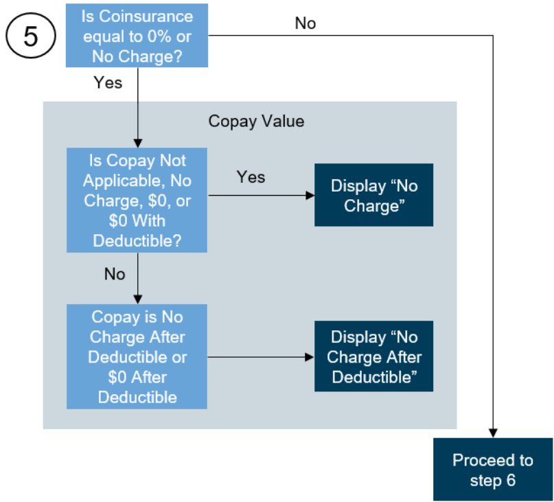
Figure 7: Copay and Coinsurance Display Process Flow Step 5
