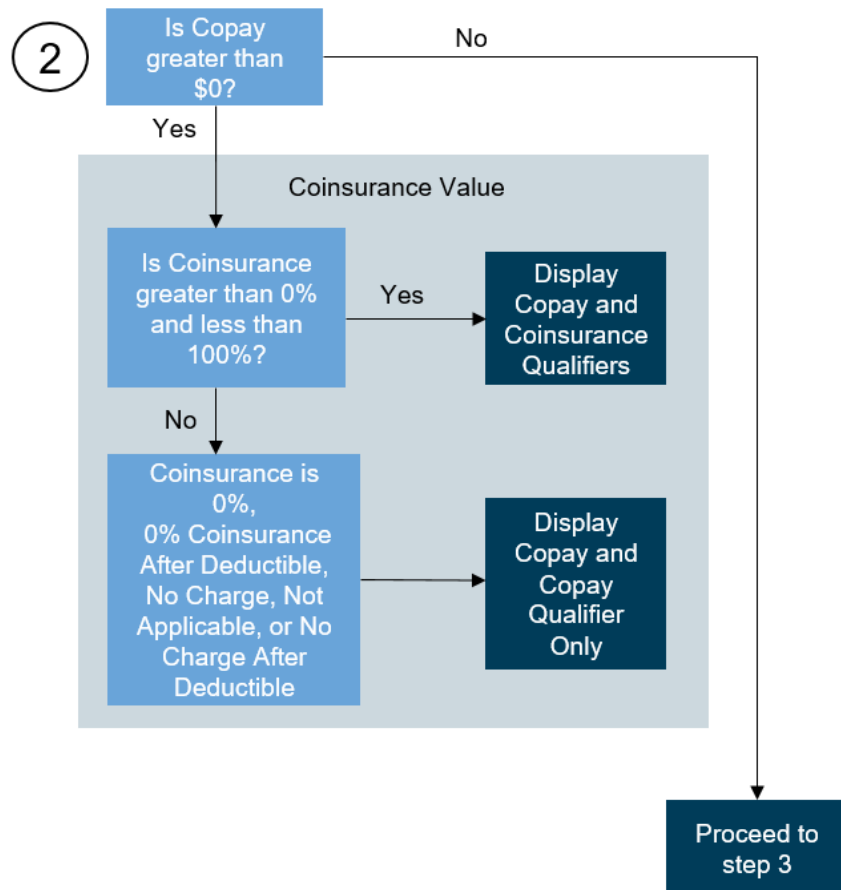
Figure 4: Copay and Coinsurance Display Process Flow Step 2
