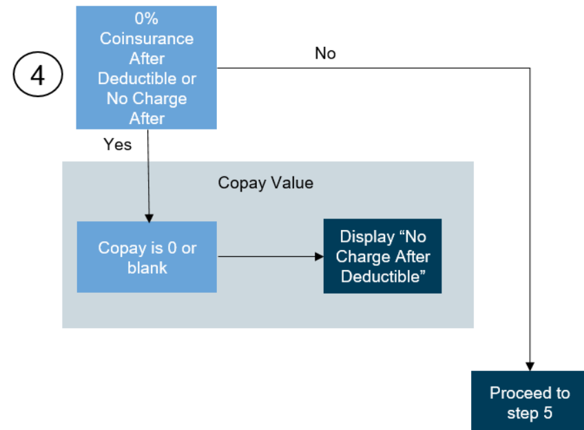
Figure 6: Copay and Coinsurance Display Process Flow Step 4
