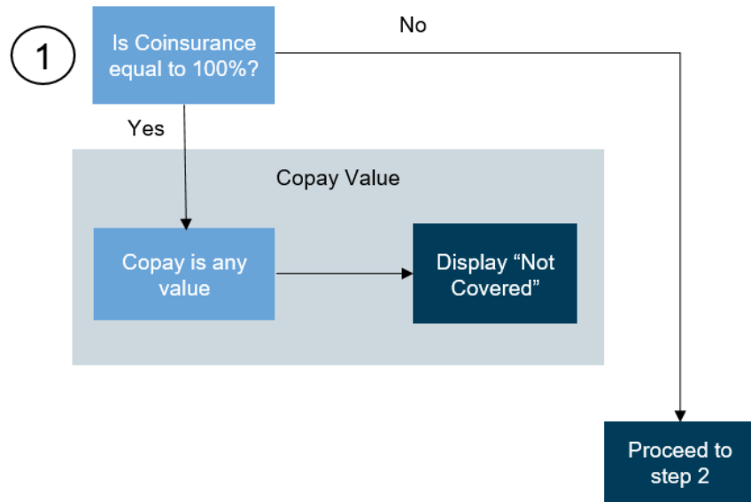
Figure 3: Copay and Coinsurance Display Process Flow Step 1
