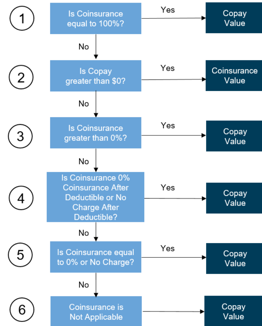
Figure 2: Coinsurance and Copay Display Logic Process Flow
