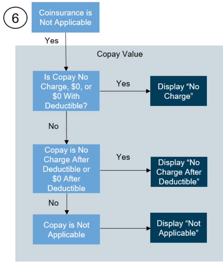
Figure 8: Copay and Coinsurance Display Process Flow Step 6
